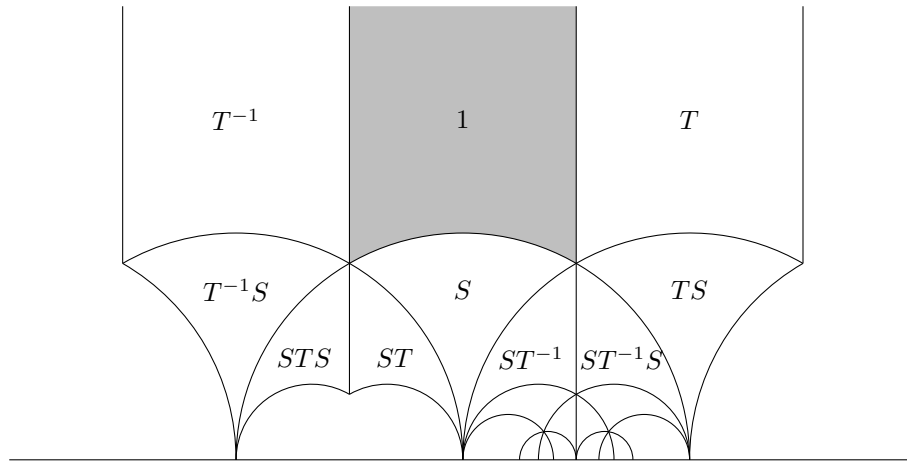
Figure 35.1.4: Tessellation of \mathbf{H}^2 into fundamental domains for \text{SL}_2(\mathbb{Z})
