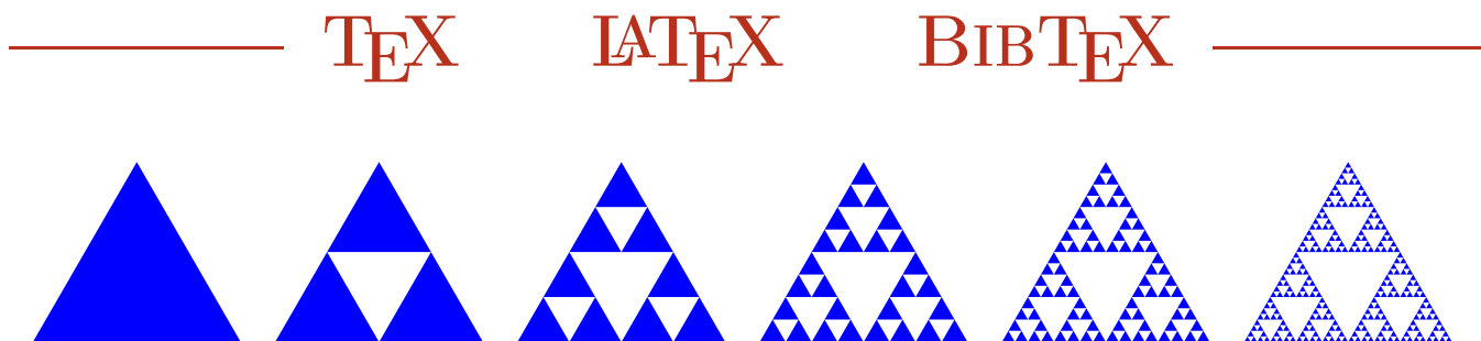
Figure 1: Sierpinski triangle created using the TikZ package
