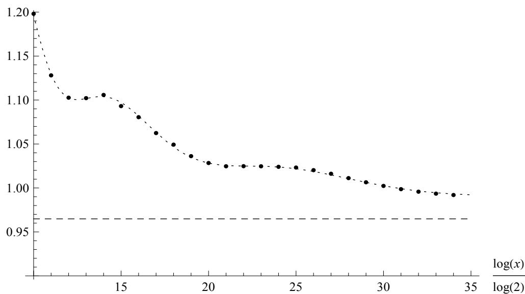
FIGURE 1. The actual values of P_\varphi(x)/(x/\log x) (dots) are well approximated by R(x) (dotted line). Also shown is \lim_{x \rightarrow \infty} R(x) (dashed line).
