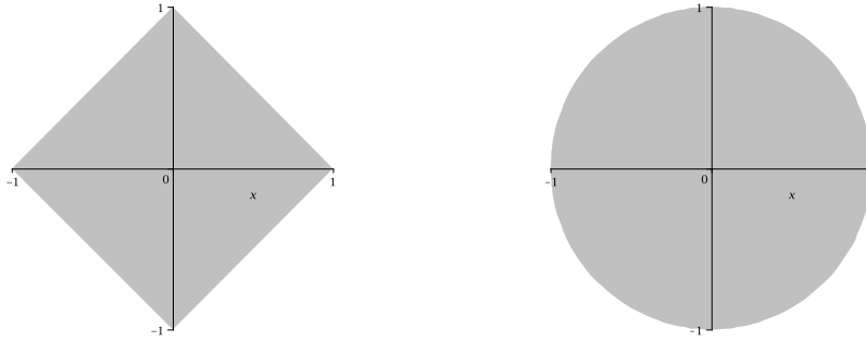
Figure 4.1: The Sets S_1 and S_2
