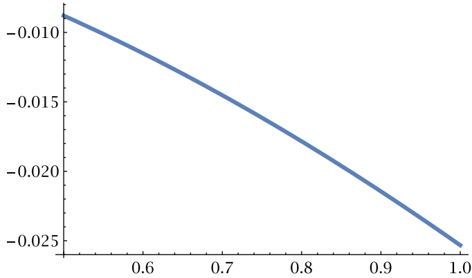
FIGURE 1. Mathematica plot of the right-hand side of (4.1) on (1/2, 1) .
