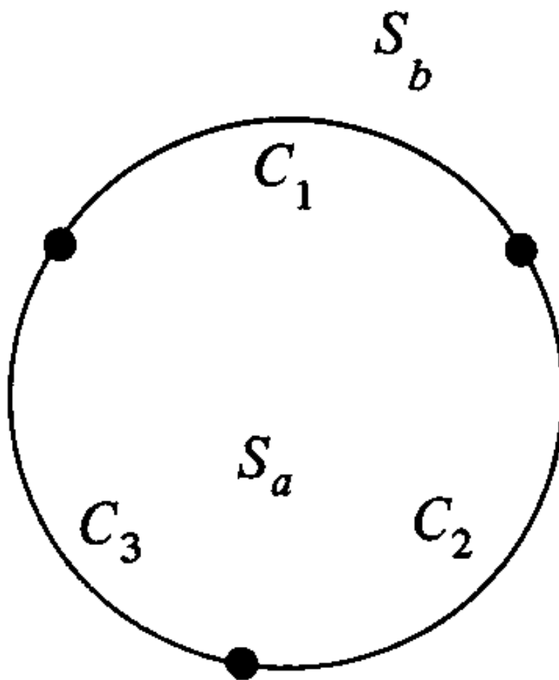
Figure 1: The punctured sphere.
