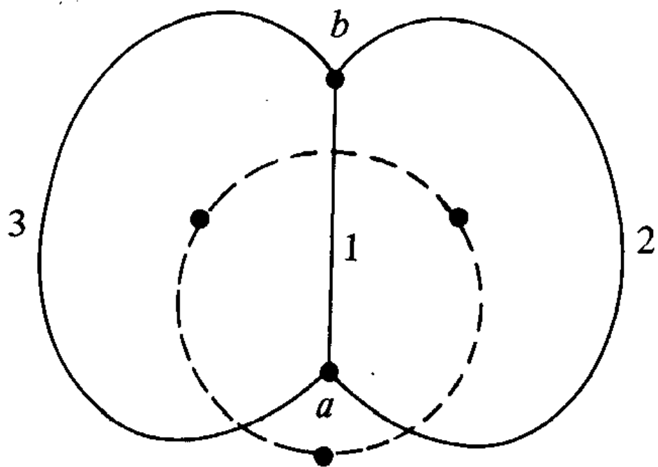
Figure 4: The dual graph.
