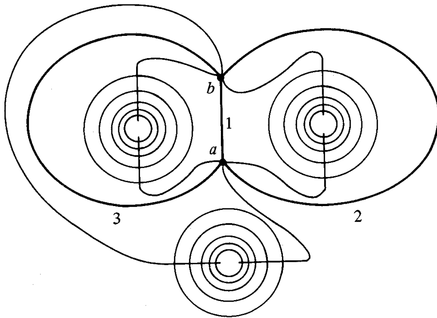
Figure 5: Quadrangulation of the punctured sphere.
