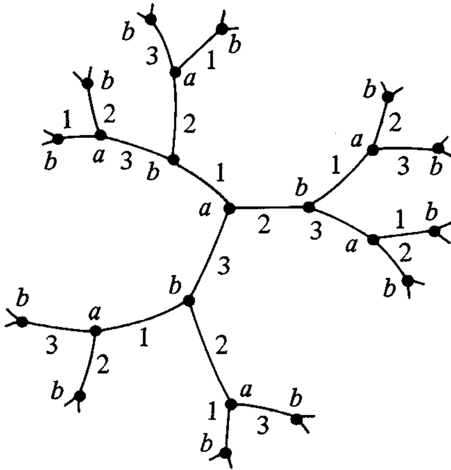
Figure 2: The universal cover of the thrice-punctured sphere.
